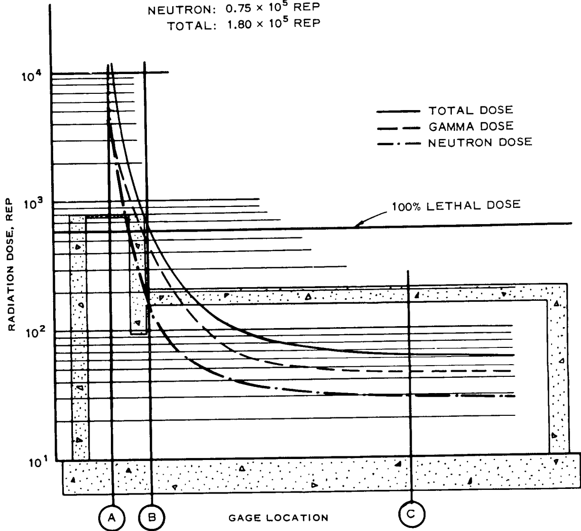
Fig. 9—Total nuclear radiation dose profile, structure 3.1a.
